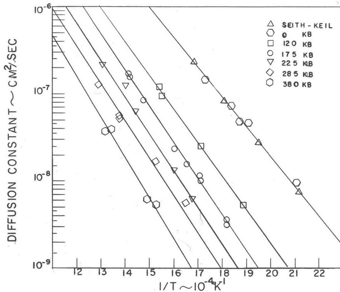
Figure 10. Plot of The Diffusion Constant versus The Reciprocal of The Anneal Temperature--Plotted in Isobars
